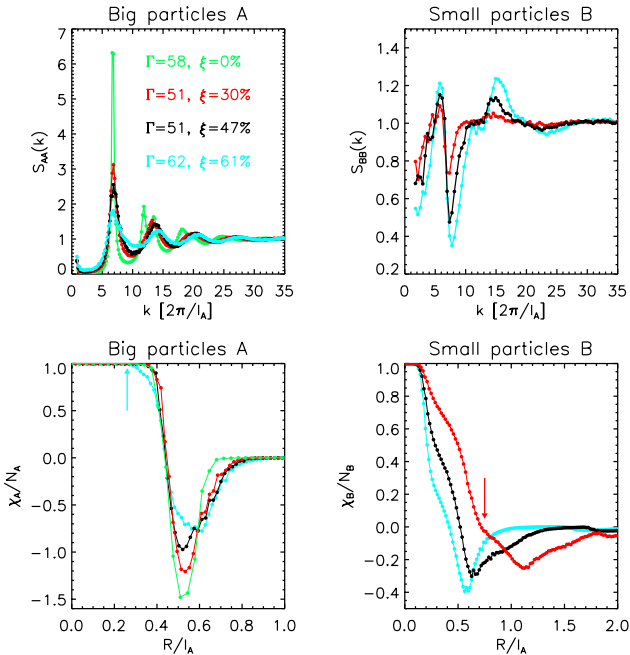
Fig. 7. (Colour on-line) Static structure factors and “Euler characteristics” of samples with comparable interaction strength \Gamma but different relative concentration \xi . Indicated values for \Gamma and \xi are valid for all graphs. Upper graphs: Static structure factors for big (left) and small particles (right). With increasing relative concentration of small particles the features of S_{BB}(k) gain more contrast, and peaks in the S_{AA}(k) are shifted slightly towards higher k -values. Lower graphs: “Euler characteristics” for big (left) and small particles (right). For decreasing \xi the minimum in \chi_B/N_B is shifted towards larger radii R . The weight of the features changes, see, e.g. , the last shoulder in the drop in \chi_B/N_B (red arrow, right plot). This shoulder results from the incorporation of isolated small particles into the network (see fig. 3) and is only visible for the lowest relative concentration \xi = 30\% (red curve) at this interaction strength \Gamma . The blue arrow in the bottom left plot marks the onset of the inter-particle connection of the big particles for the sample with highest relative concentration \xi = 61\% . The onset is shifted to a lower value R compared to the other curves.
